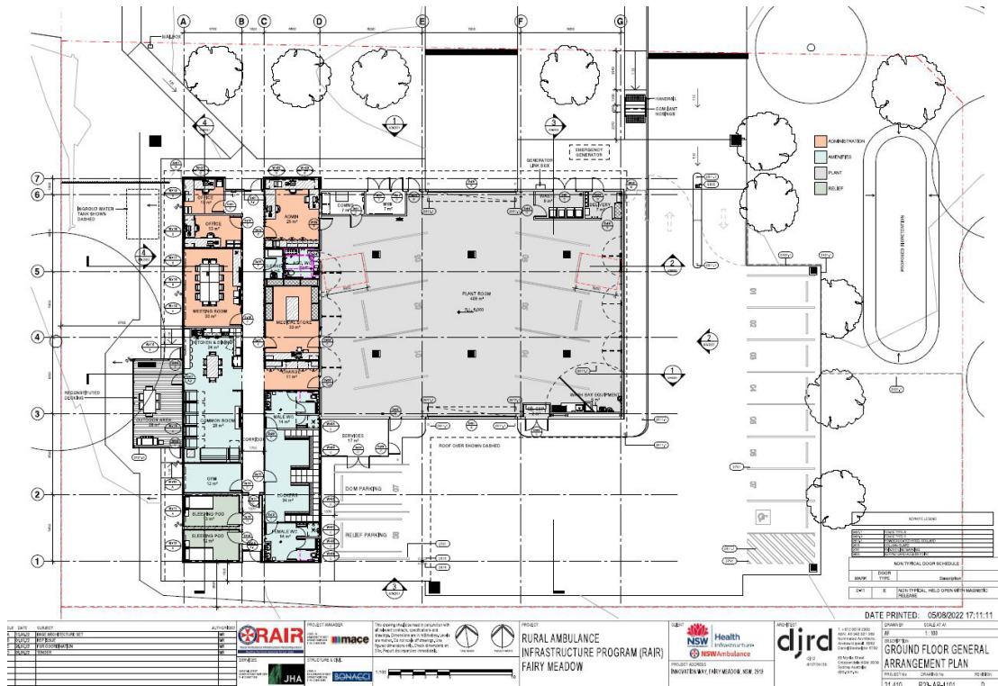
Figure 8. Excerpt of Ground Floor General Arrangement Plan (R23-AR-1101, Rev D). (djrd, 5 August 2022).
